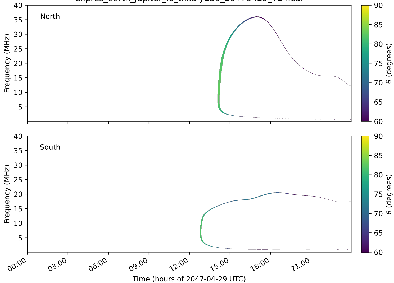
expres_earth_jupiter_io_txka-y235_20470429_v14.cdf
