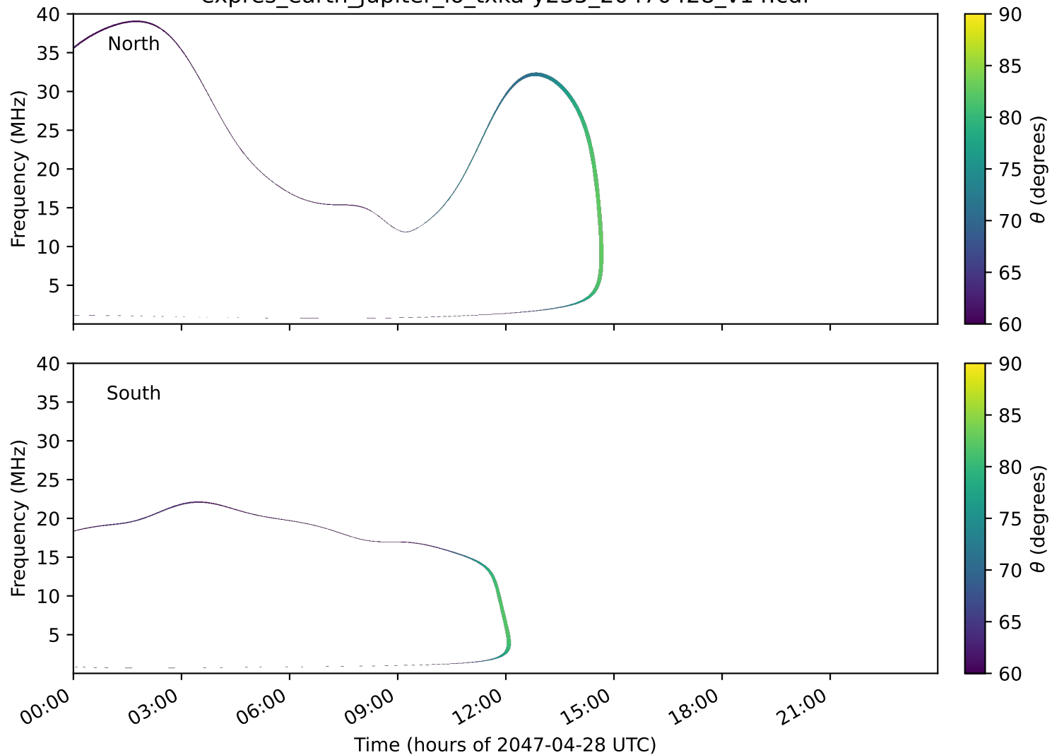
expres_earth_jupiter_io_txka-y235_20470428_v14.cdf
