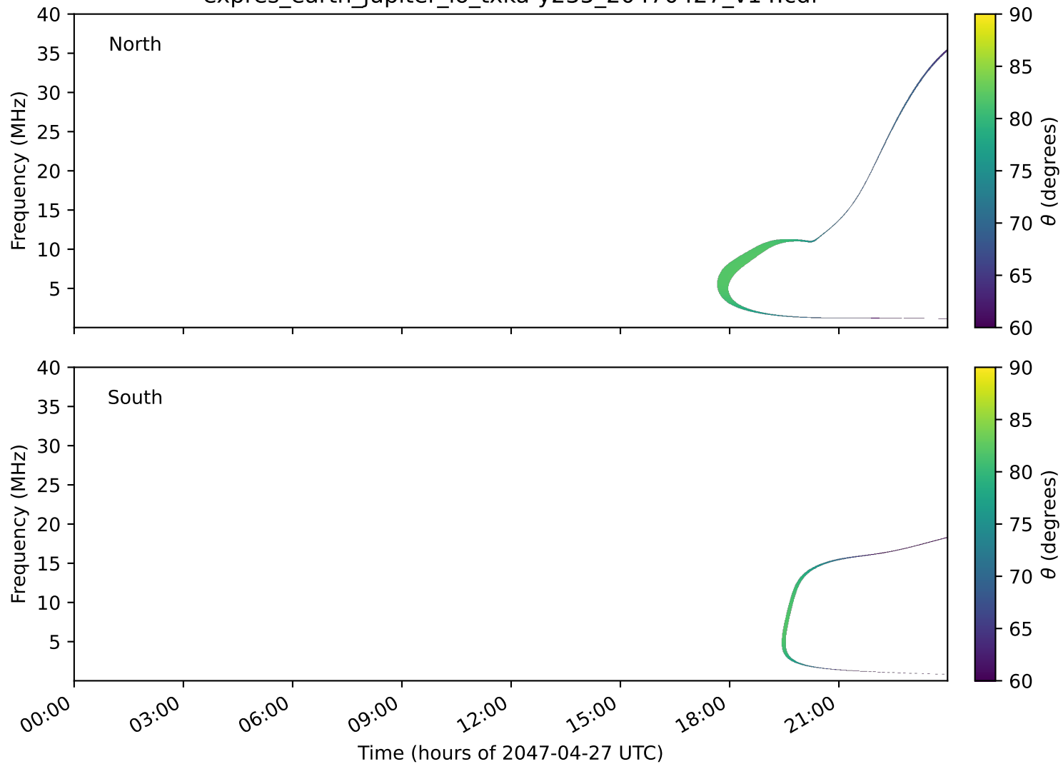
expres_earth_jupiter_io_txka-y235_20470427_v14.cdf
