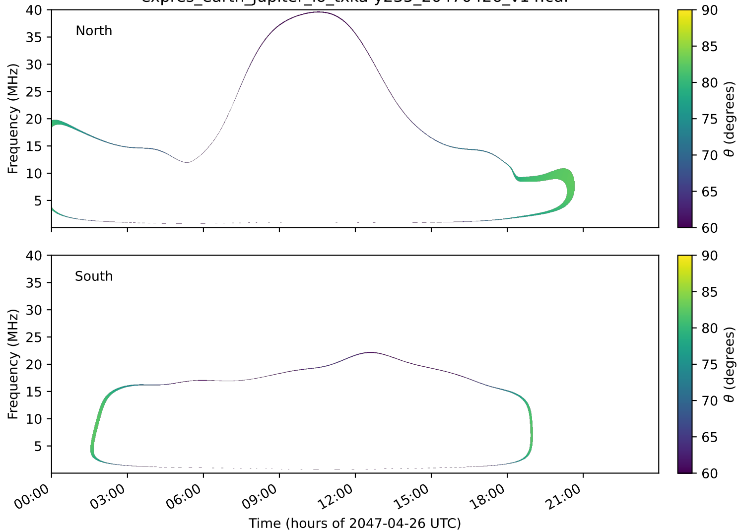
expres_earth_jupiter_io_txka-y235_20470426_v14.cdf
