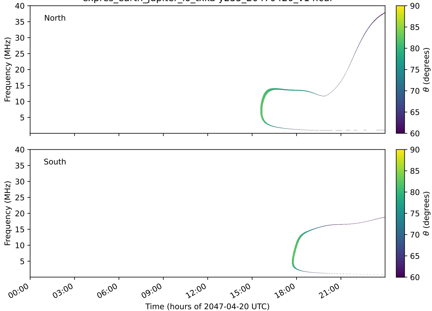
expres_earth_jupiter_io_txka-y235_20470420_v14.cdf
