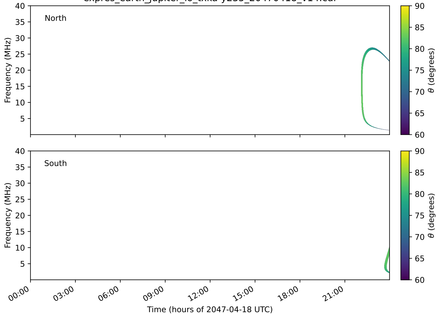
expres_earth_jupiter_io_txka-y235_20470418_v14.cdf
