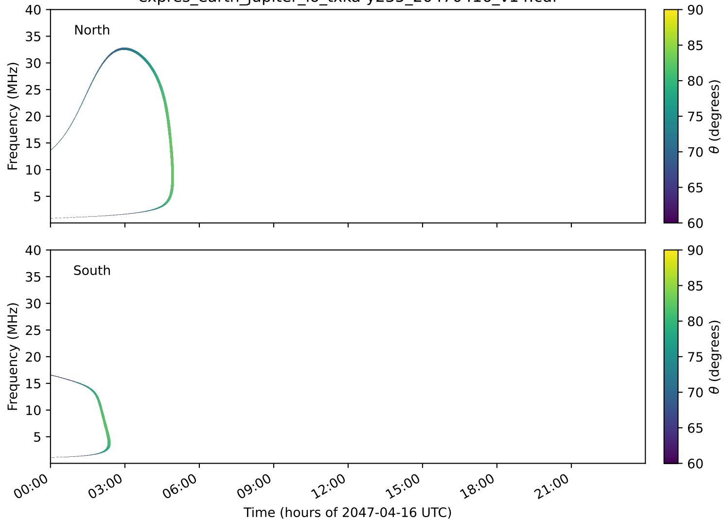
expres_earth_jupiter_io_txka-y235_20470416_v14.cdf
