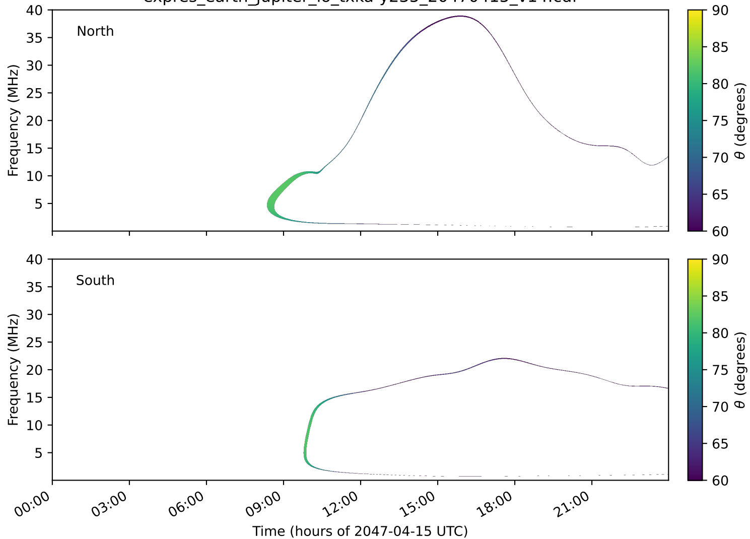
expres_earth_jupiter_io_txka-y235_20470415_v14.cdf
