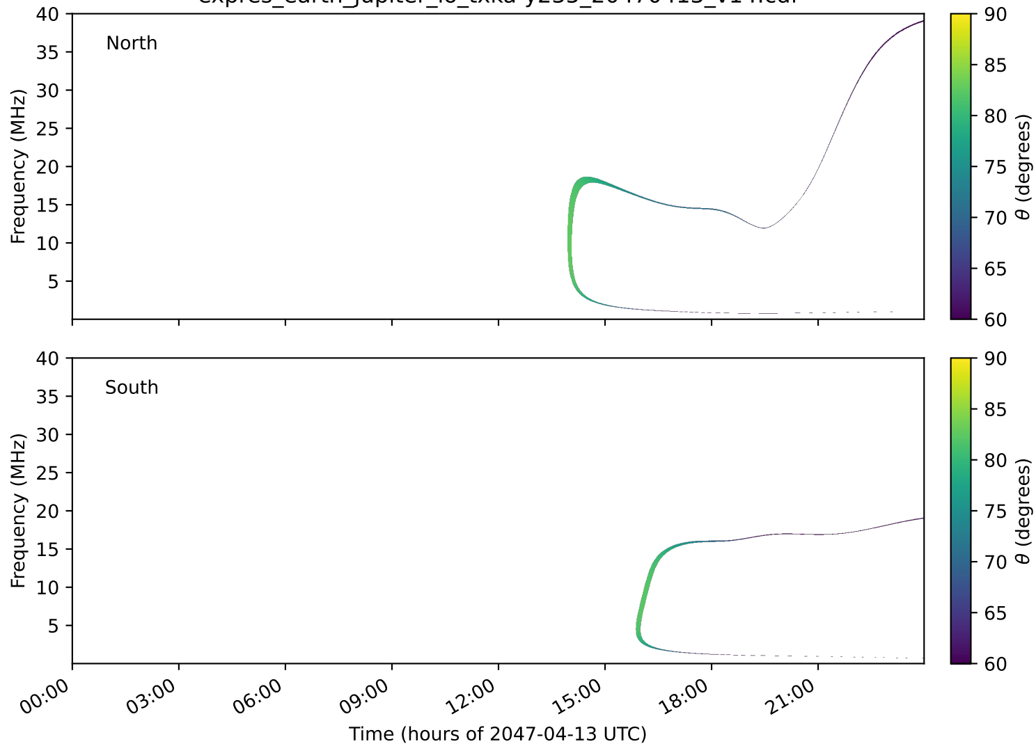
expres_earth_jupiter_io_txka-y235_20470413_v14.cdf
