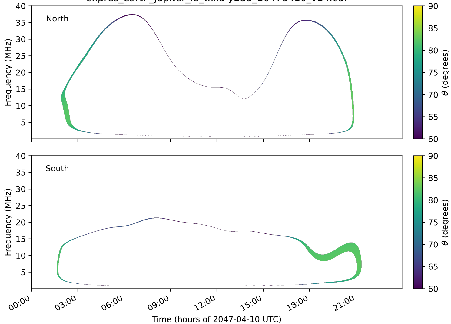
expres_earth_jupiter_io_txka-y235_20470410_v14.cdf
