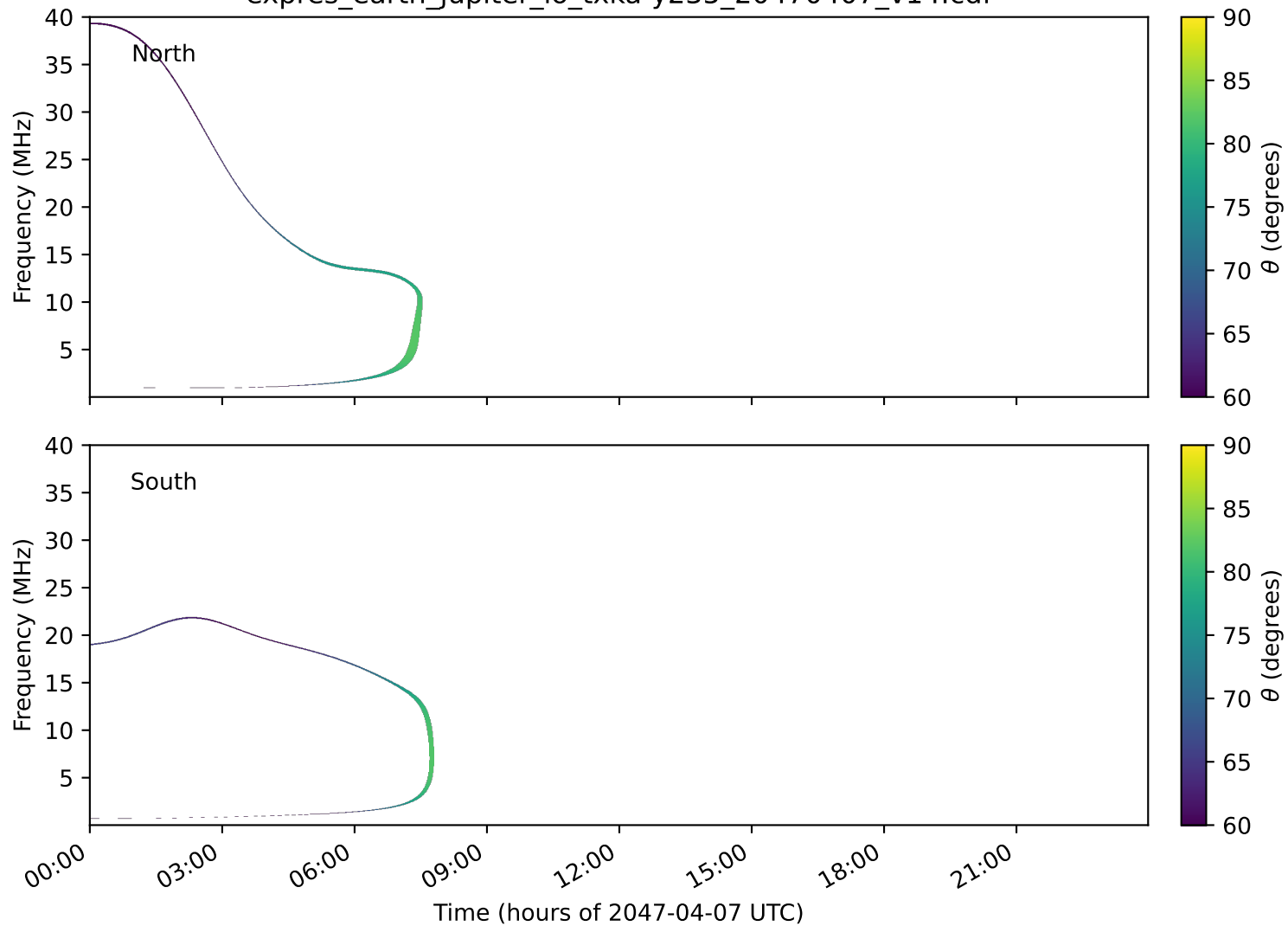
expres_earth_jupiter_io_txka-y235_20470407_v14.cdf
