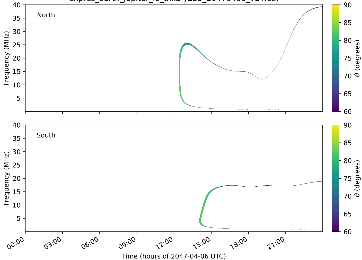
expres_earth_jupiter_io_txka-y235_20470406_v14.cdf
