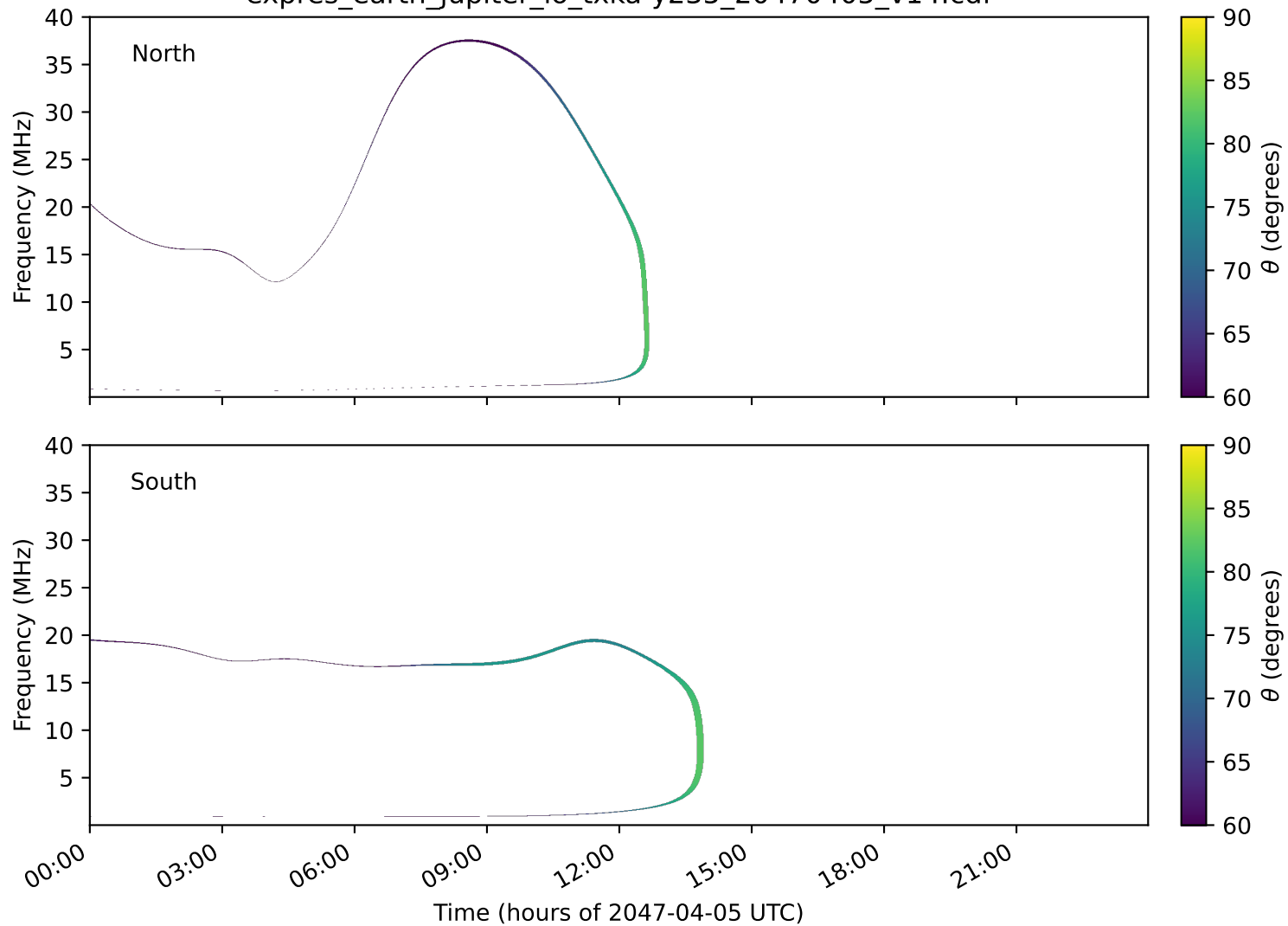
expres_earth_jupiter_io_txka-y235_20470405_v14.cdf
