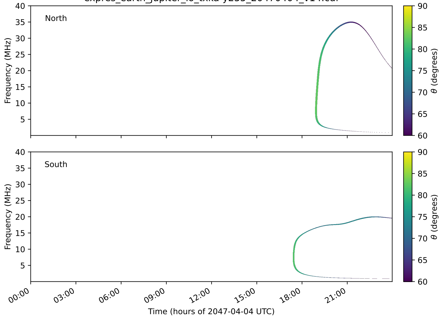
expres_earth_jupiter_io_txka-y235_20470404_v14.cdf
