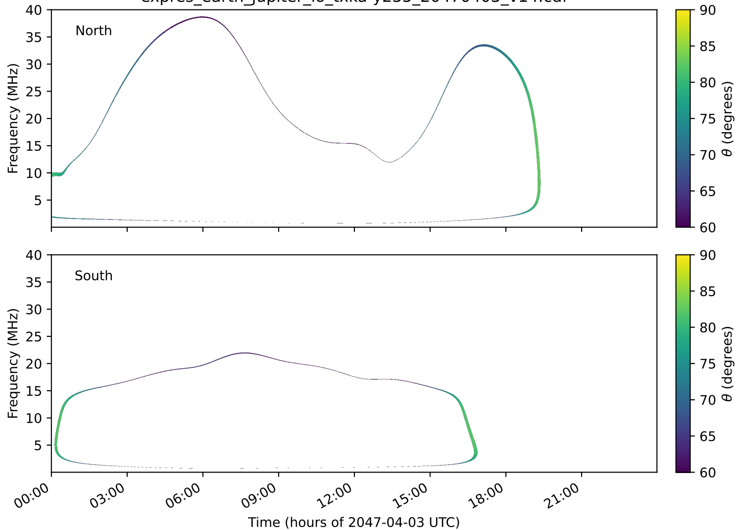
expres_earth_jupiter_io_txka-y235_20470403_v14.cdf
