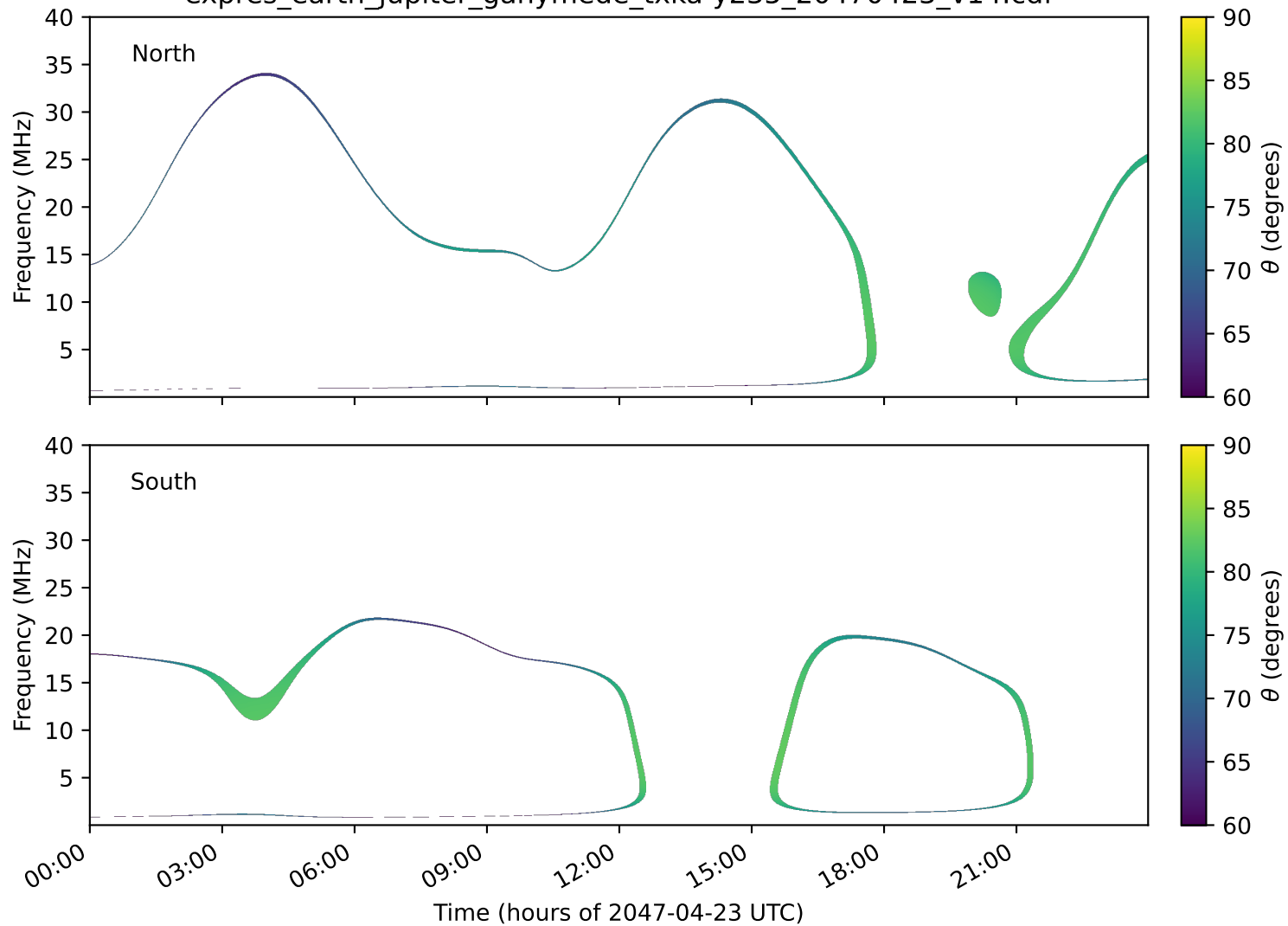
expres_earth_jupiter_ganymede_txka-y235_20470423_v14.cdf
