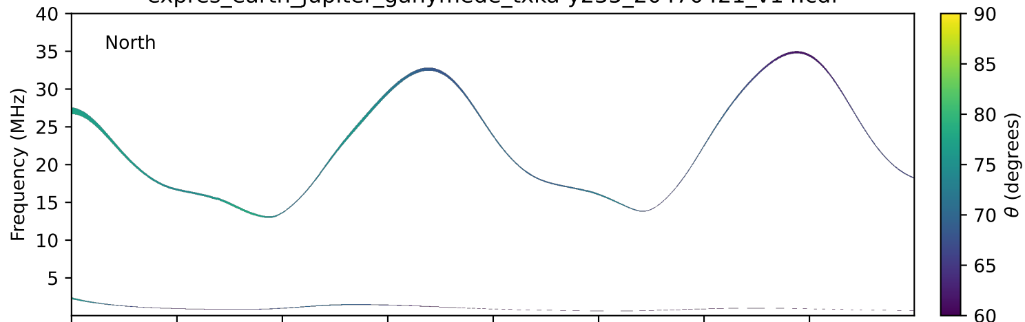
expres_earth_jupiter_ganymede_txka-y235_20470421_v14.cdf
