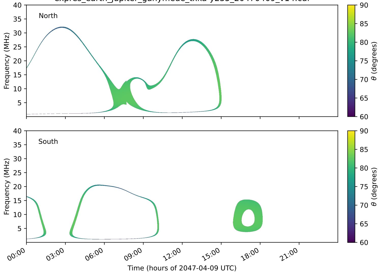
expres_earth_jupiter_ganymede_txka-y235_20470409_v14.cdf
