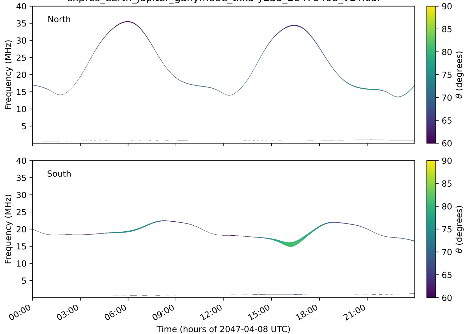
expres_earth_jupiter_ganymede_txka-y235_20470408_v14.cdf
