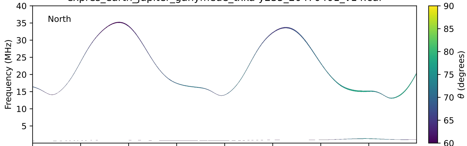
expres_earth_jupiter_ganymede_txka-y235_20470401_v14.cdf
