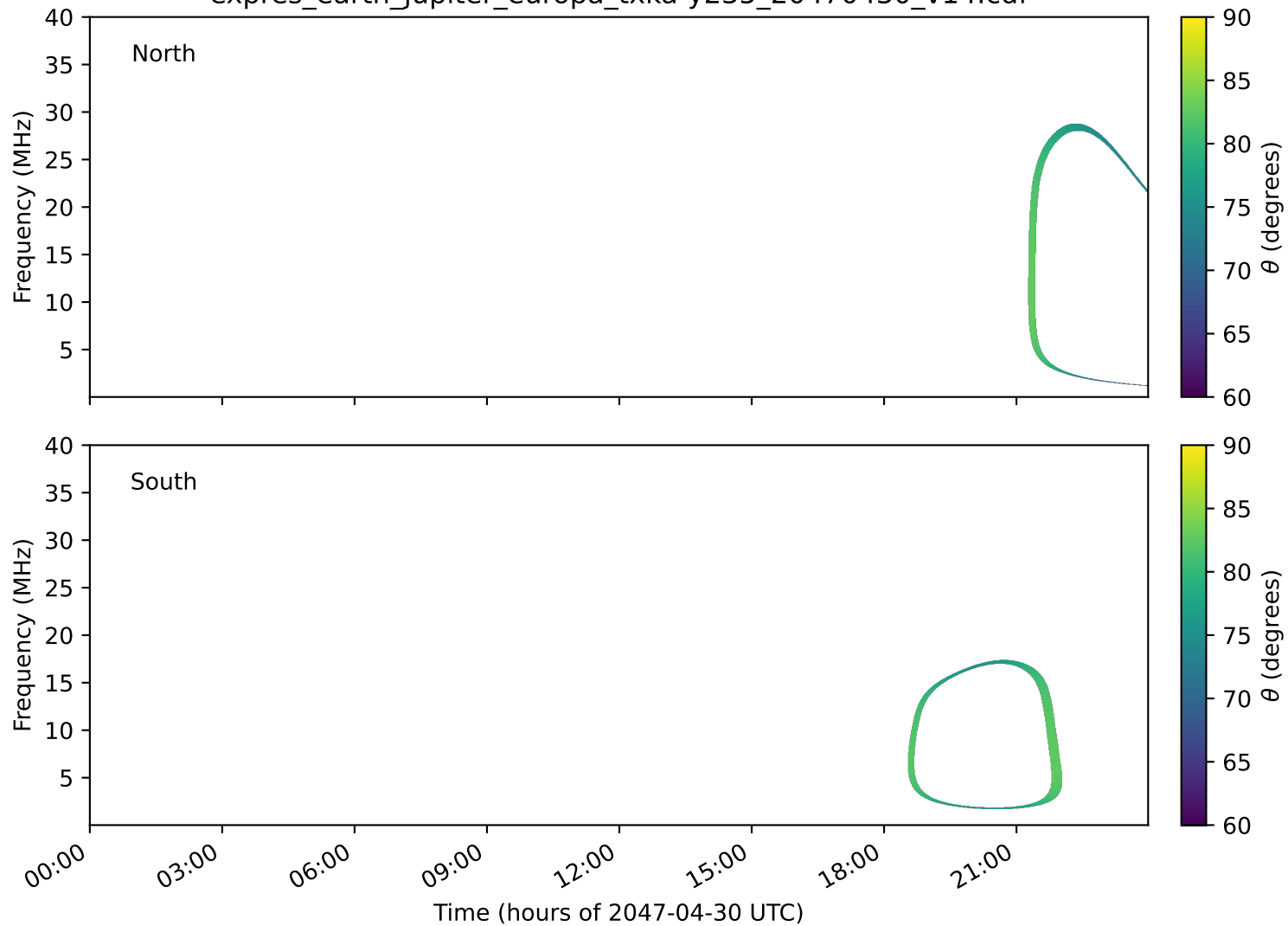
expres_earth_jupiter_europa_txka-y235_20470430_v14.cdf
