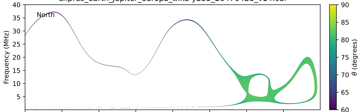
expres_earth_jupiter_europa_txka-y235_20470428_v14.cdf
