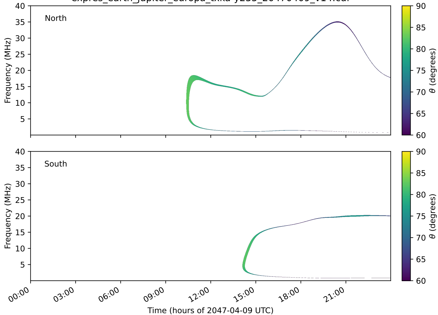
expres_earth_jupiter_europa_txka-y235_20470409_v14.cdf
