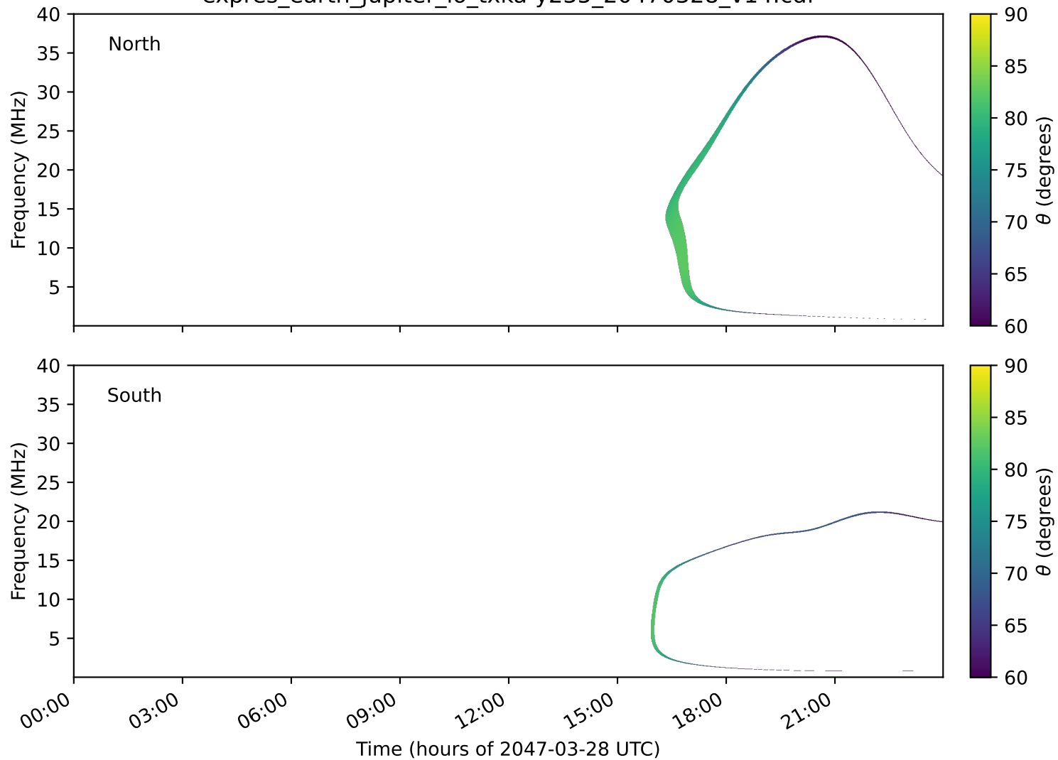
expres_earth_jupiter_io_txka-y235_20470328_v14.cdf
