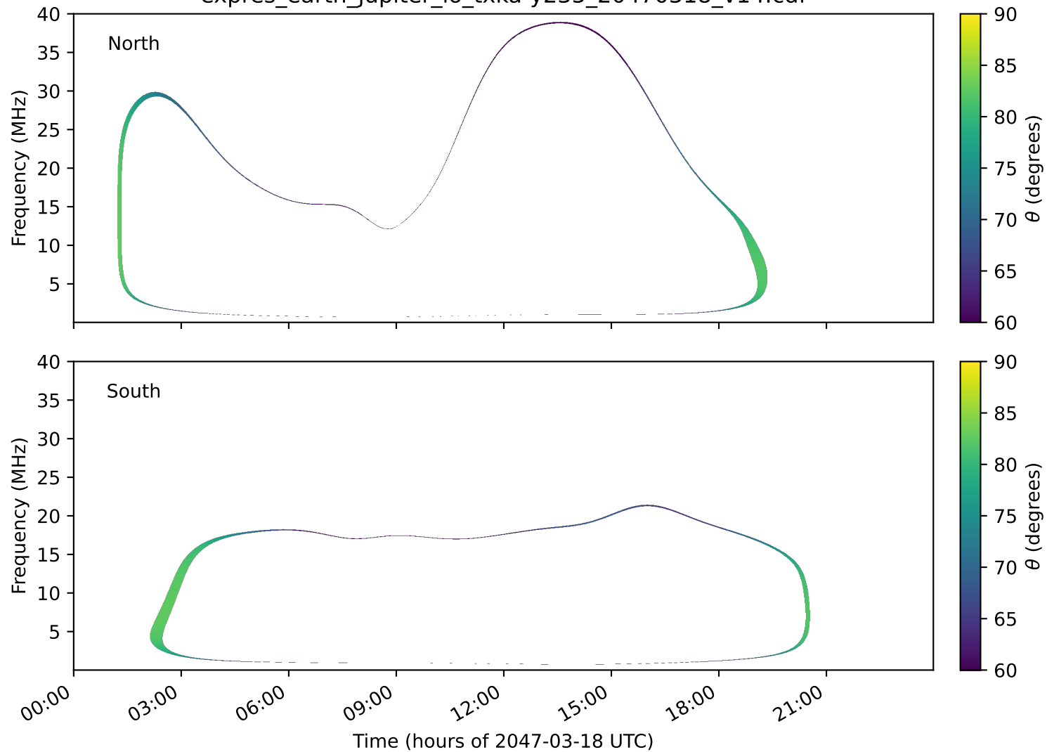
expres_earth_jupiter_io_txka-y235_20470318_v14.cdf
