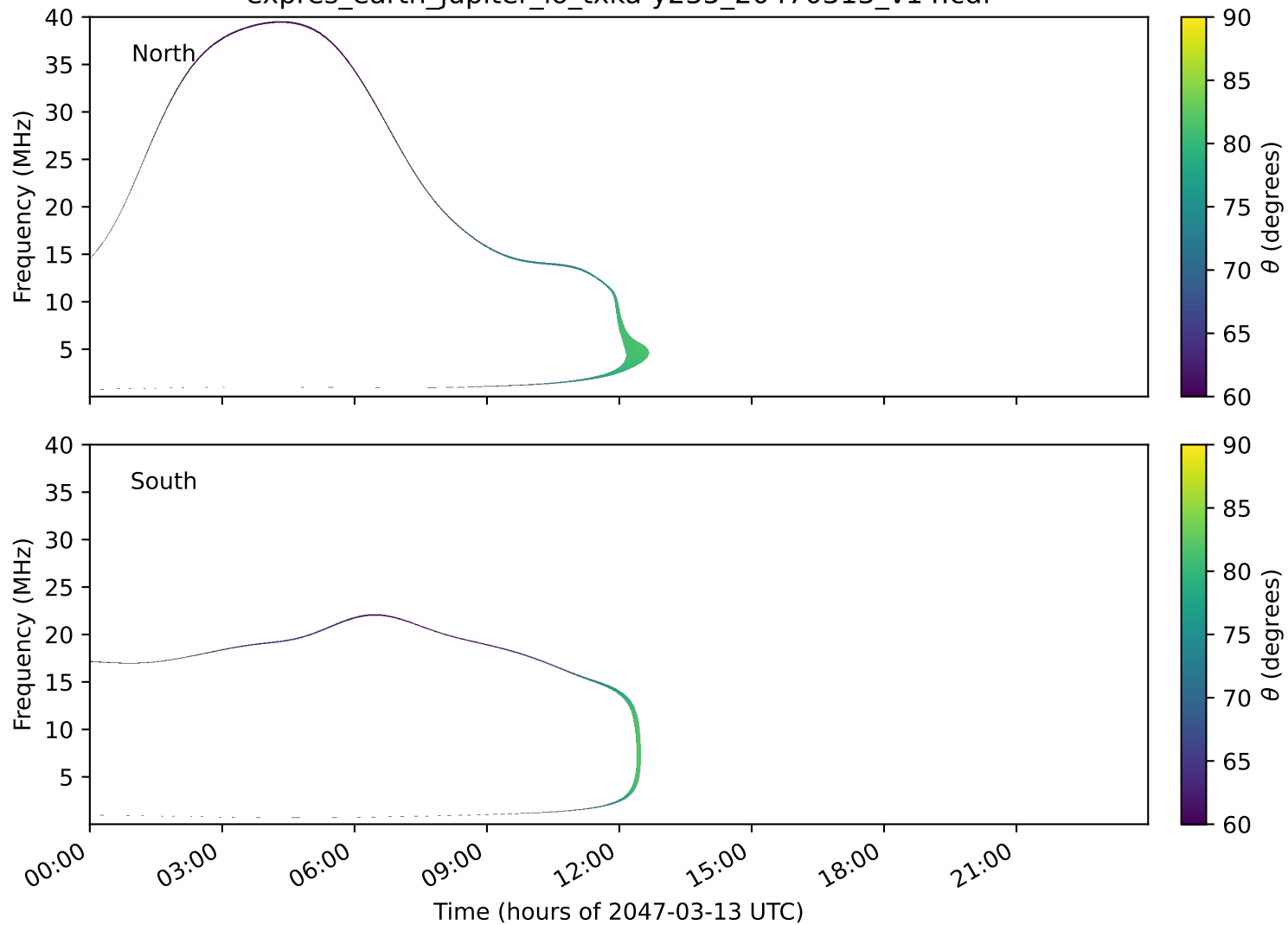
expres_earth_jupiter_io_txka-y235_20470313_v14.cdf
