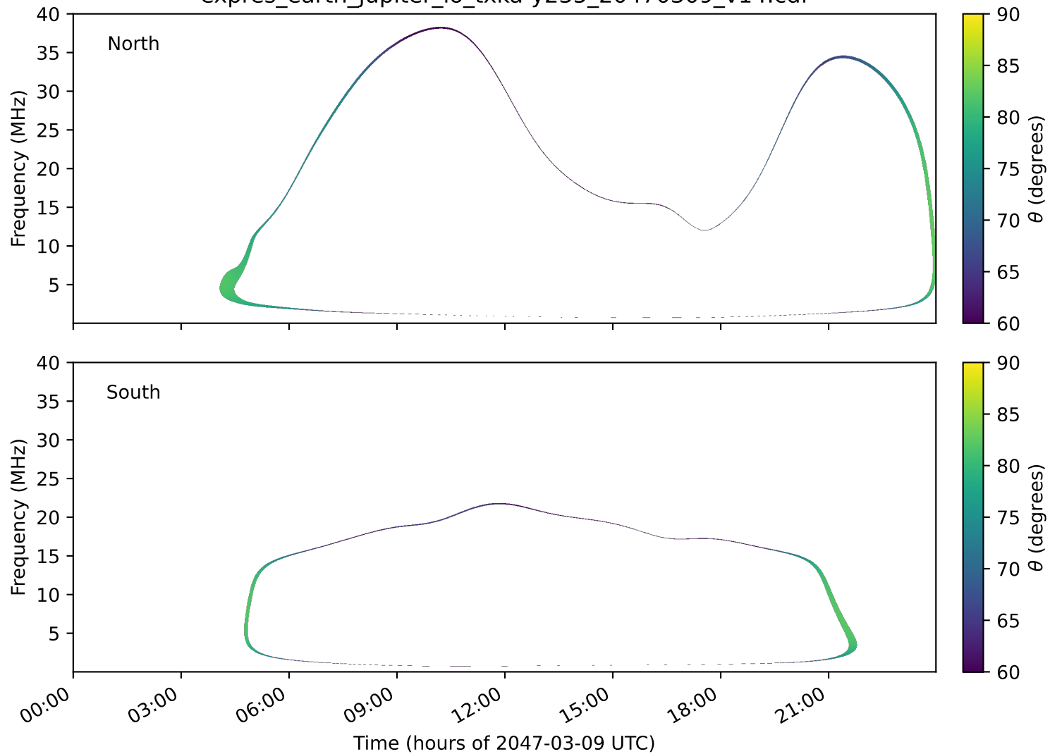
expres_earth_jupiter_io_txka-y235_20470309_v14.cdf
