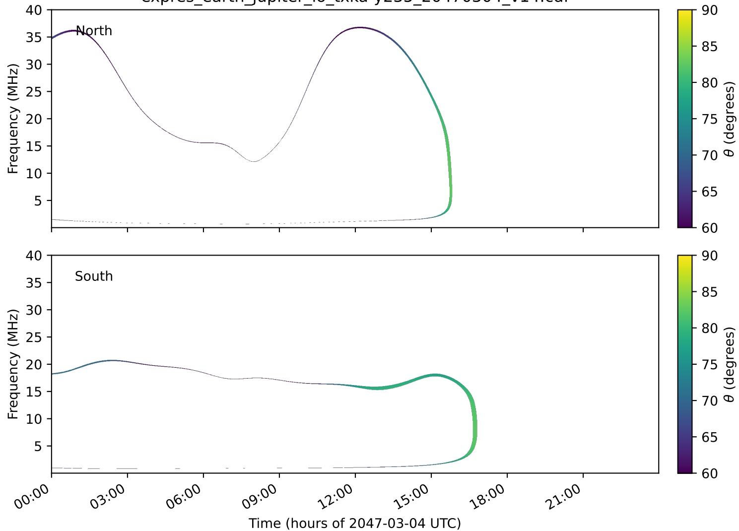
expres_earth_jupiter_io_txka-y235_20470304_v14.cdf
