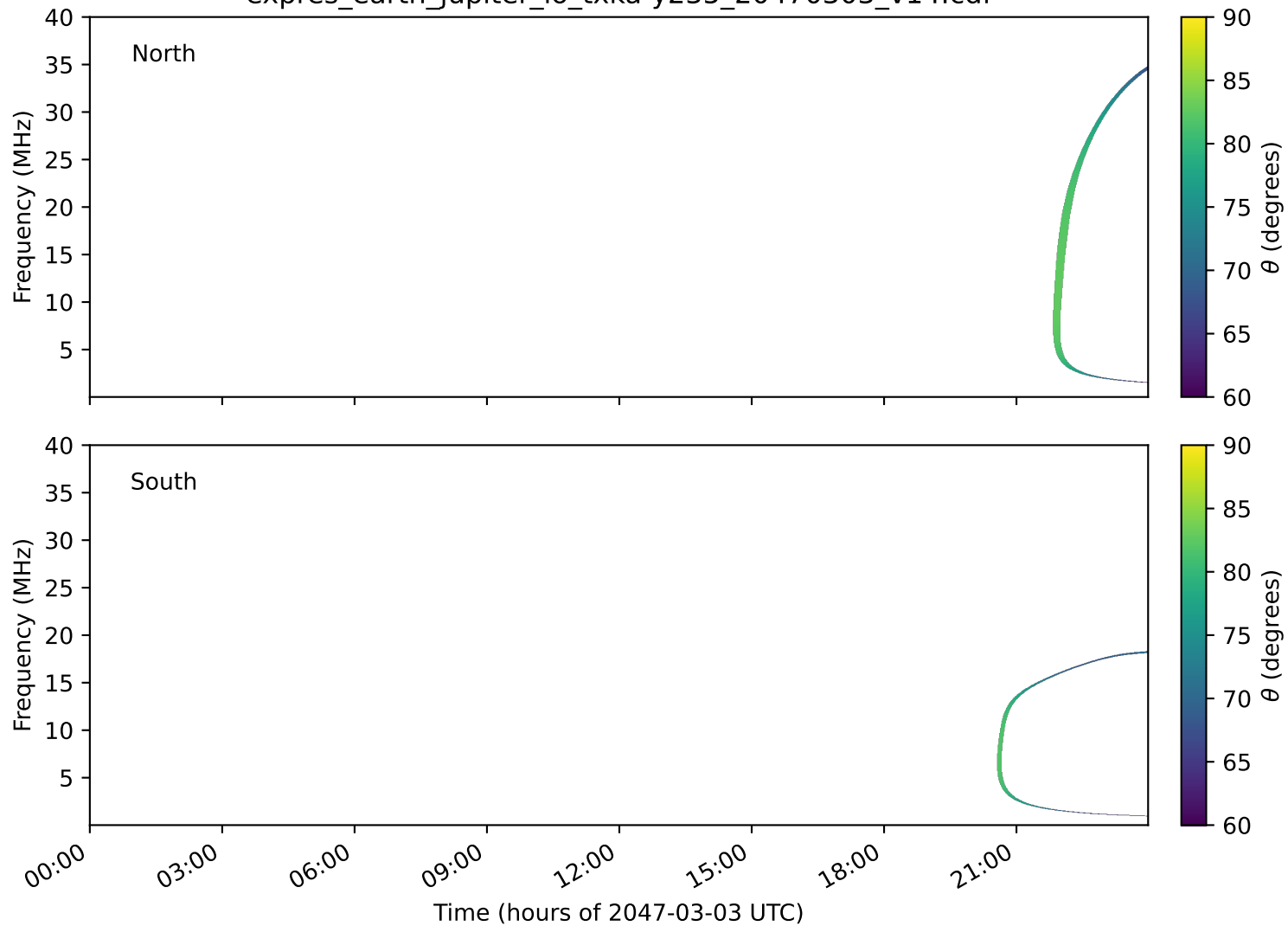
expres_earth_jupiter_io_txka-y235_20470303_v14.cdf
