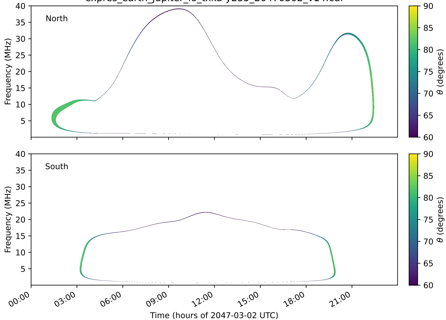
expres_earth_jupiter_io_txka-y235_20470302_v14.cdf
