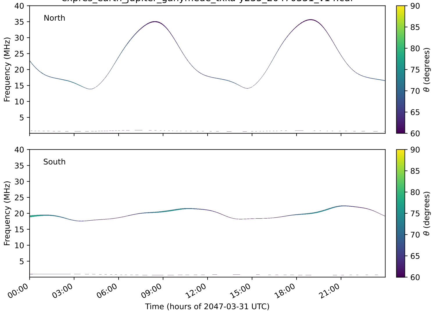
expres_earth_jupiter_ganymede_txka-y235_20470331_v14.cdf
