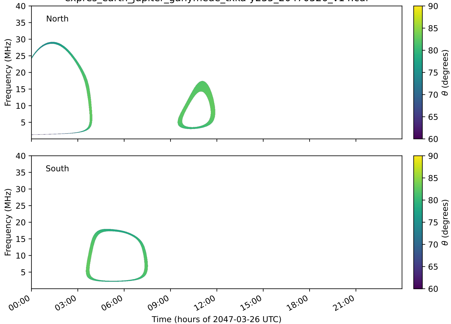
expres_earth_jupiter_ganymede_txka-y235_20470326_v14.cdf
