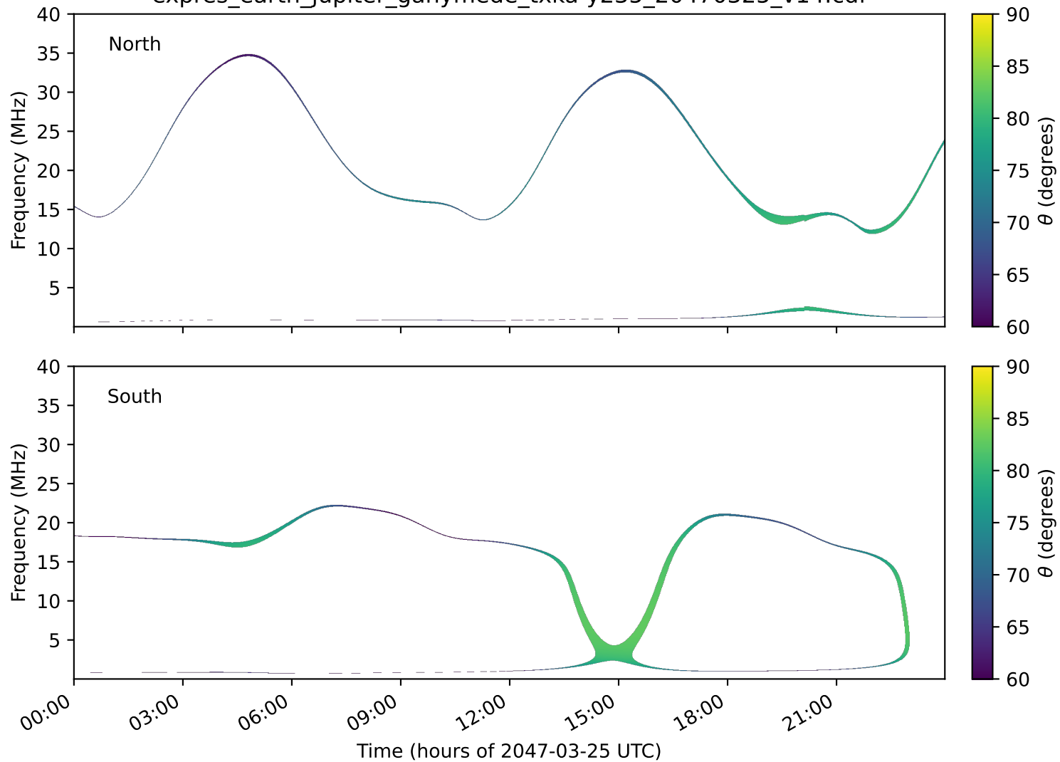
expres_earth_jupiter_ganymede_txka-y235_20470325_v14.cdf
