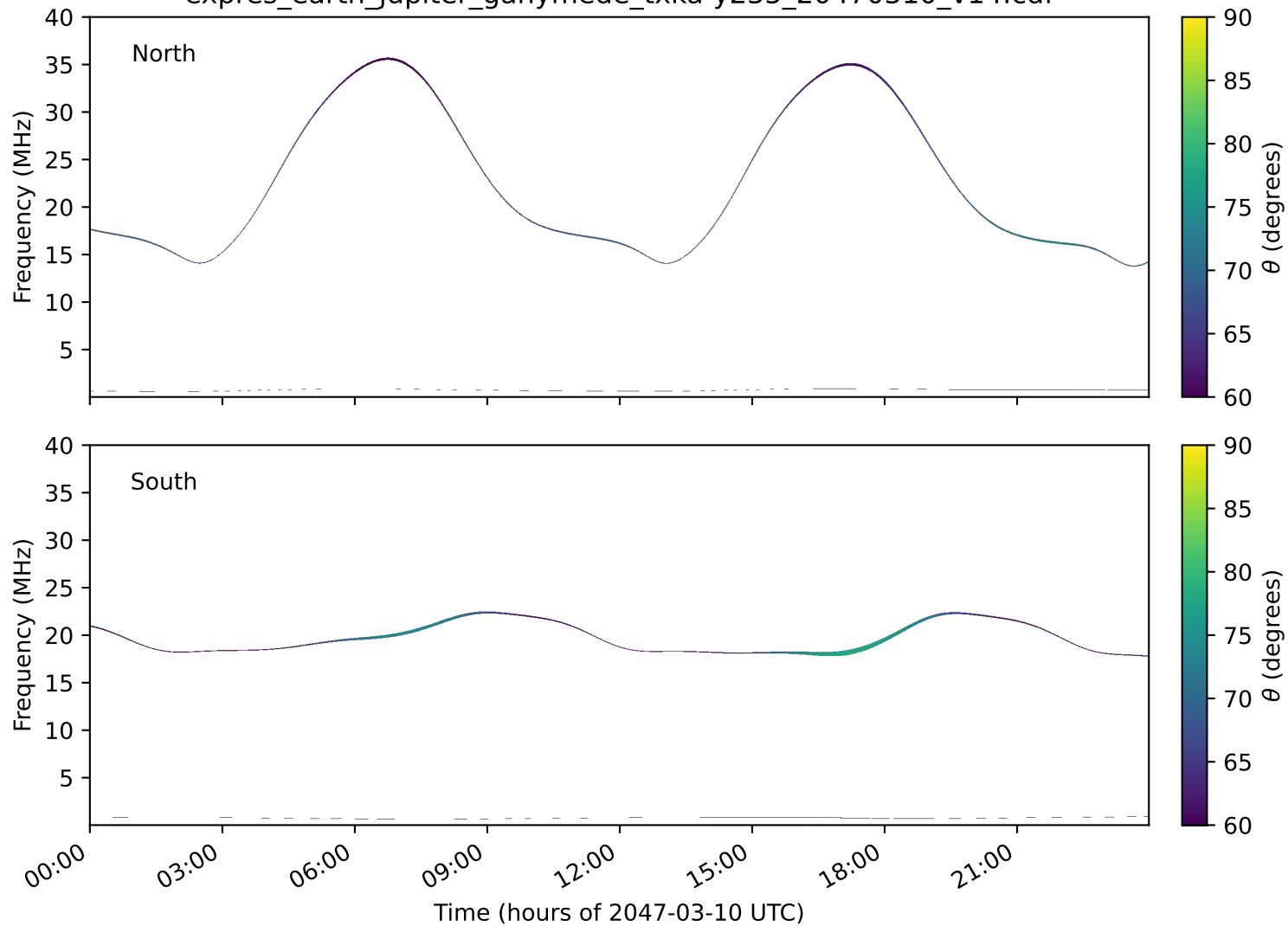
expres_earth_jupiter_ganymede_txka-y235_20470310_v14.cdf
