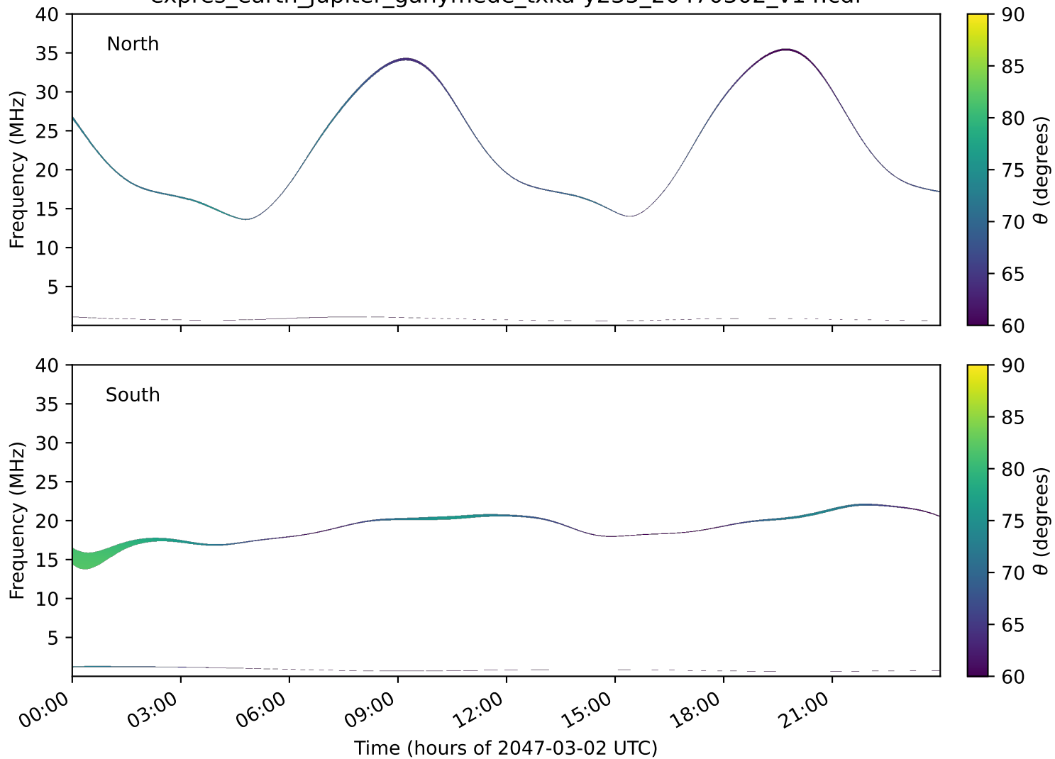
expres_earth_jupiter_ganymede_txka-y235_20470302_v14.cdf
