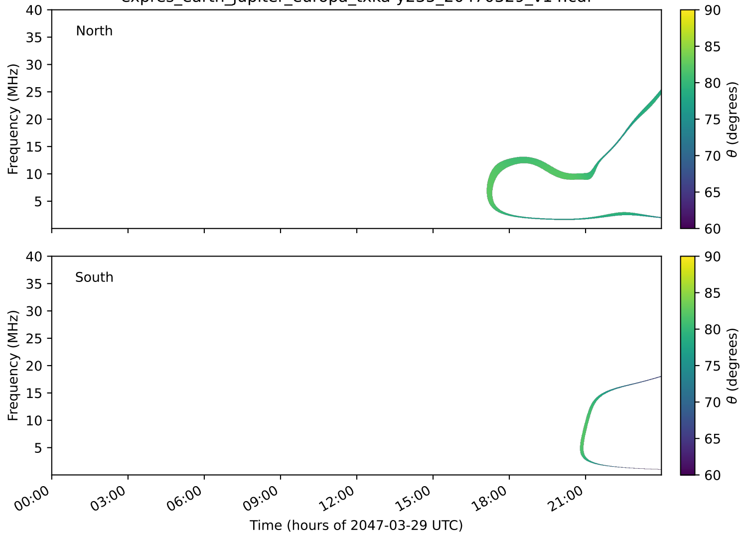
expres_earth_jupiter_europa_txka-y235_20470329_v14.cdf
