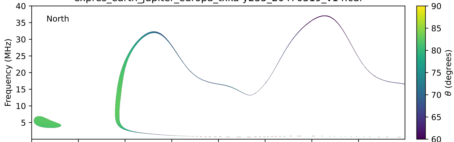
expres_earth_jupiter_europa_txka-y235_20470319_v14.cdf
