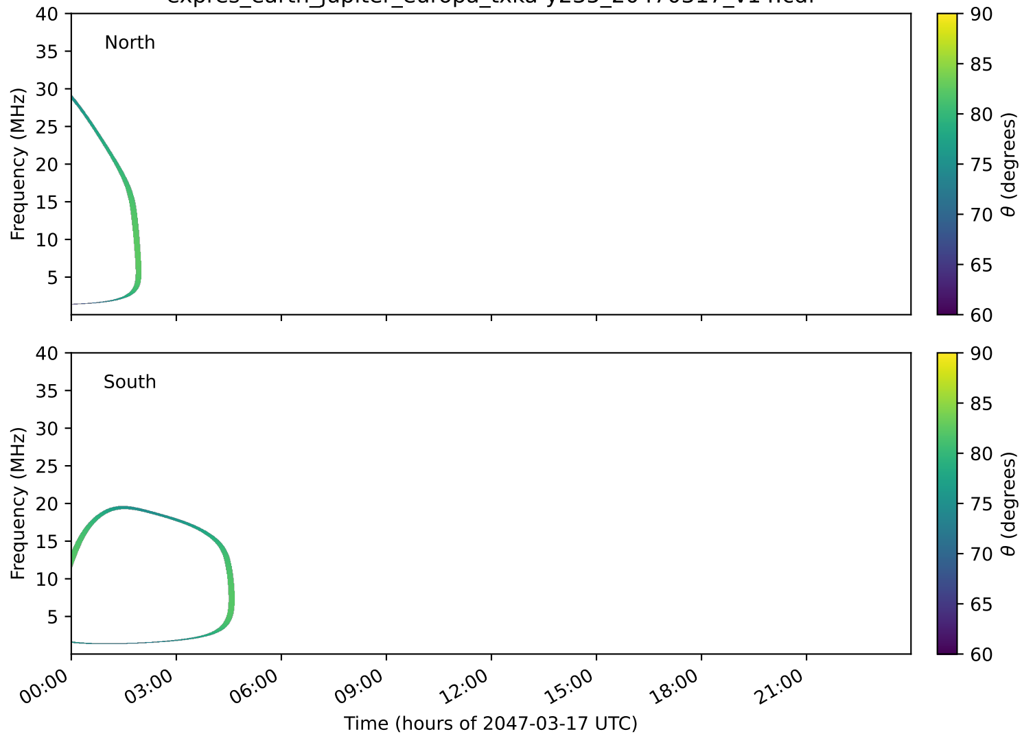
expres_earth_jupiter_europa_txka-y235_20470317_v14.cdf
