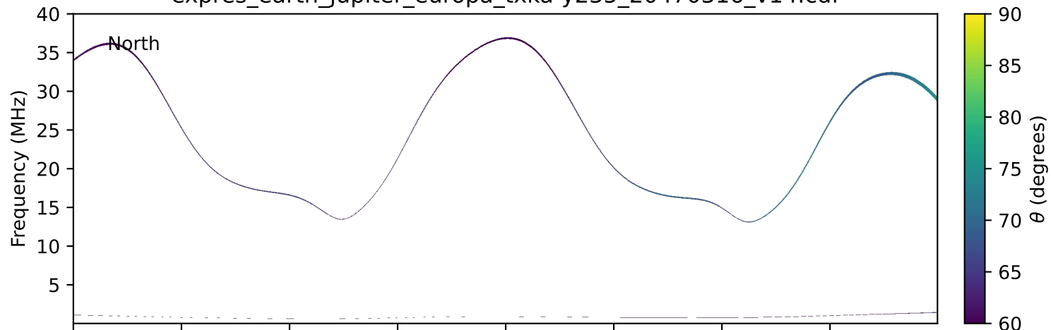
expres_earth_jupiter_europa_txka-y235_20470316_v14.cdf
