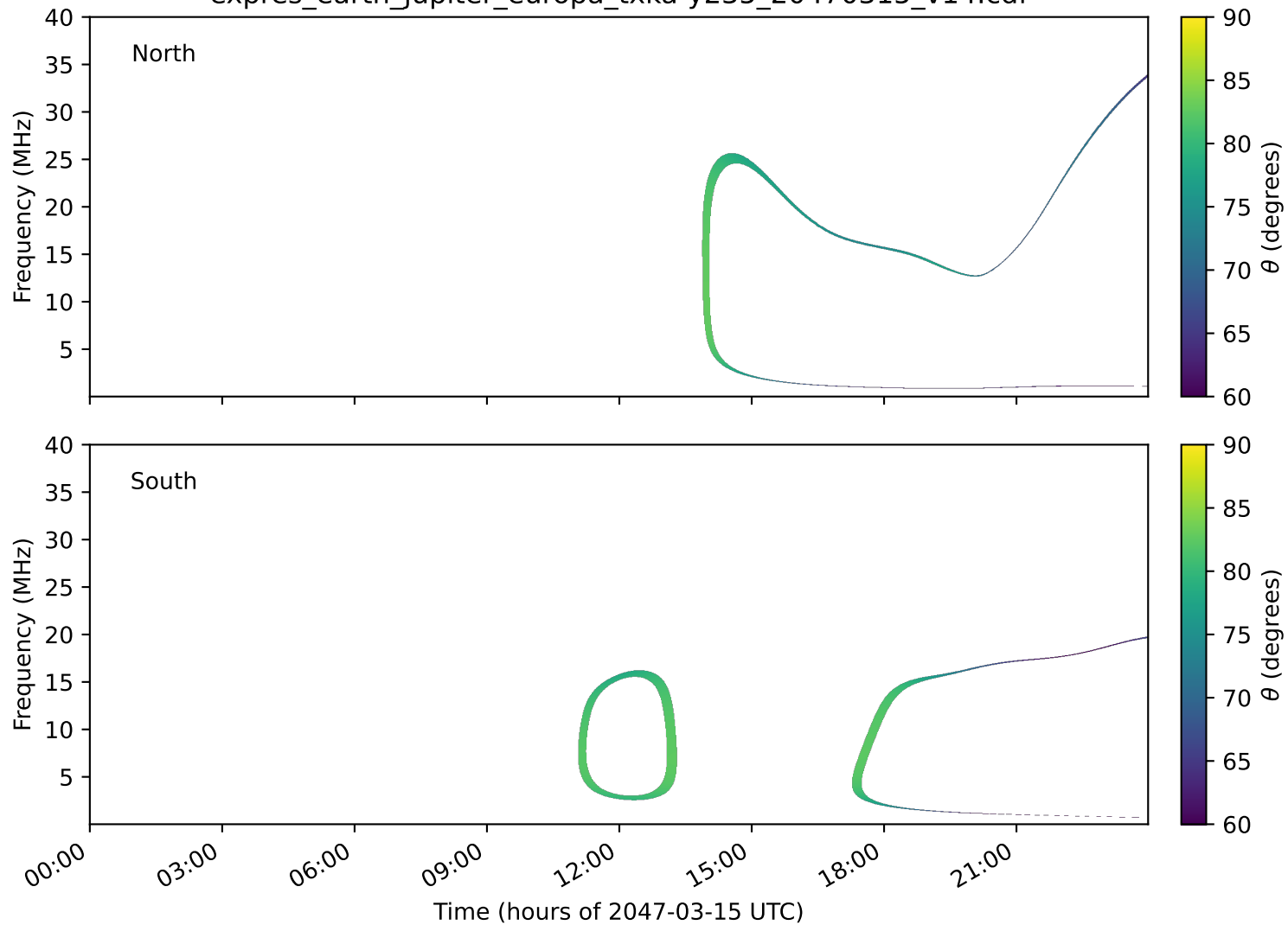
expres_earth_jupiter_europa_txka-y235_20470315_v14.cdf
