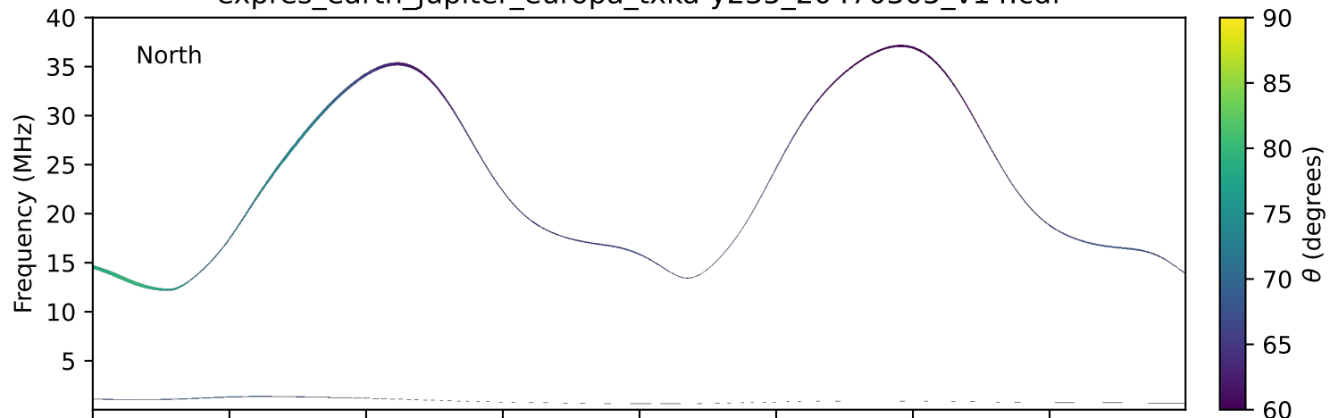
expres_earth_jupiter_europa_txka-y235_20470305_v14.cdf
