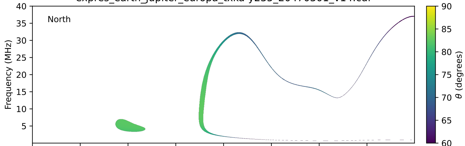
expres_earth_jupiter_europa_txka-y235_20470301_v14.cdf
