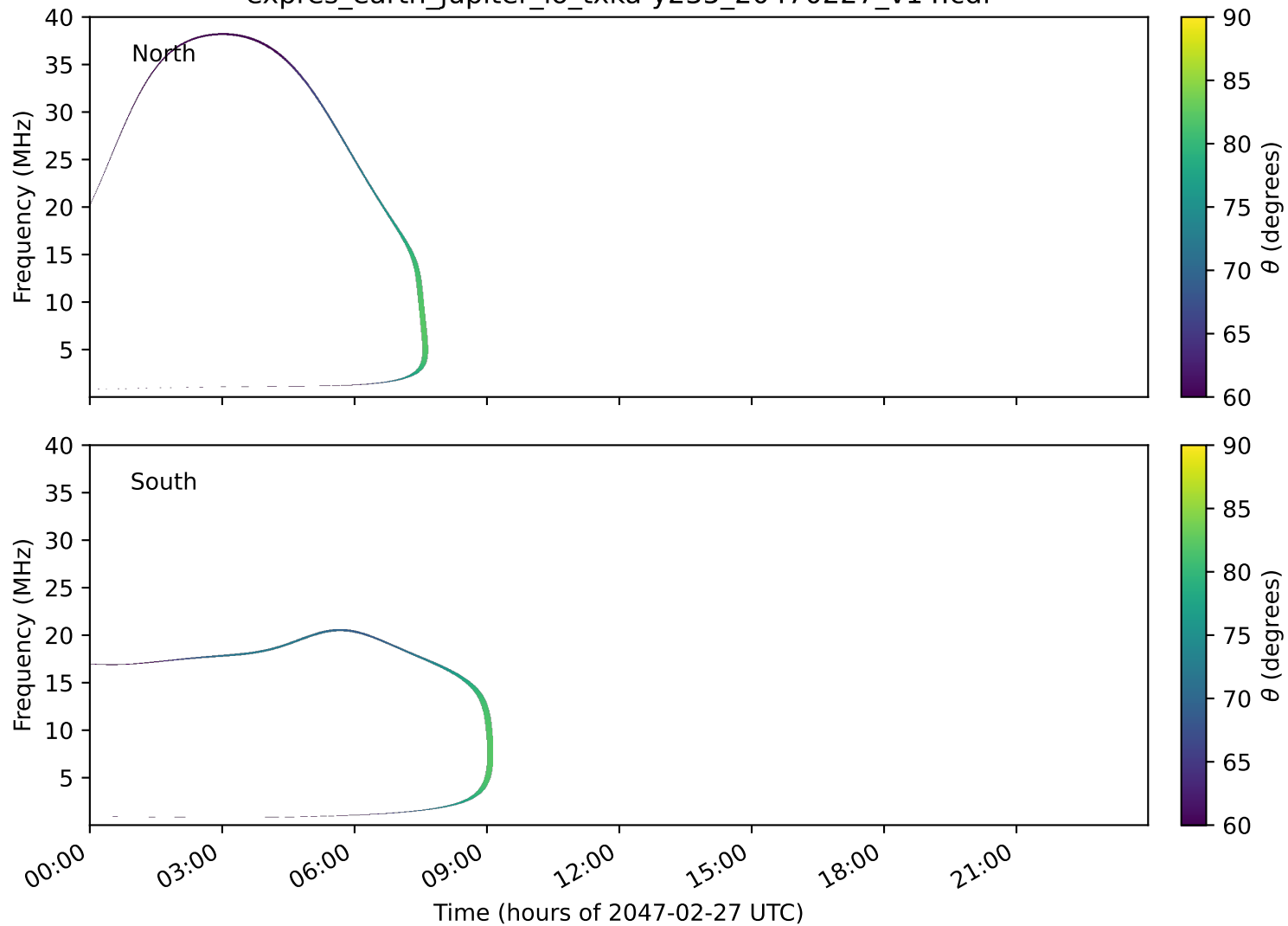
expres_earth_jupiter_io_txka-y235_20470227_v14.cdf
