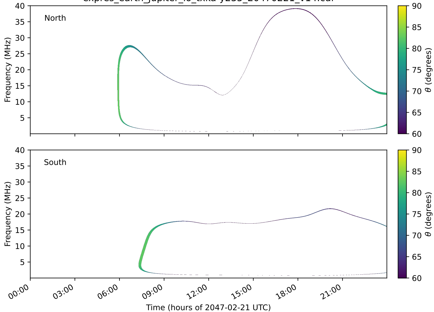
expres_earth_jupiter_io_txka-y235_20470221_v14.cdf
