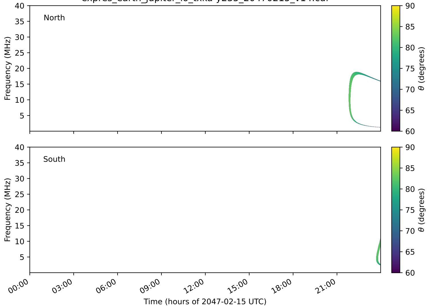
expres_earth_jupiter_io_txka-y235_20470215_v14.cdf
