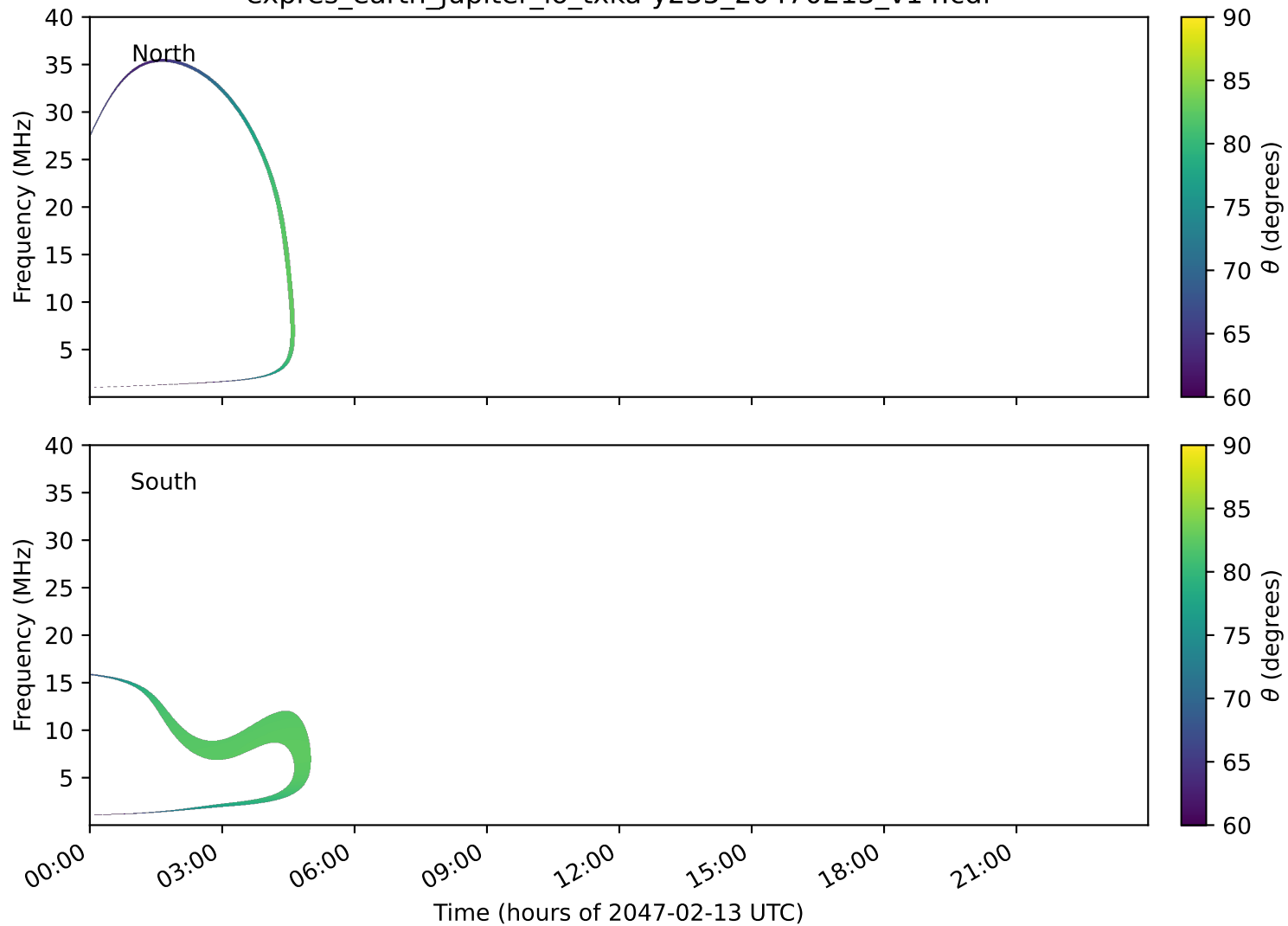
expres_earth_jupiter_io_txka-y235_20470213_v14.cdf
