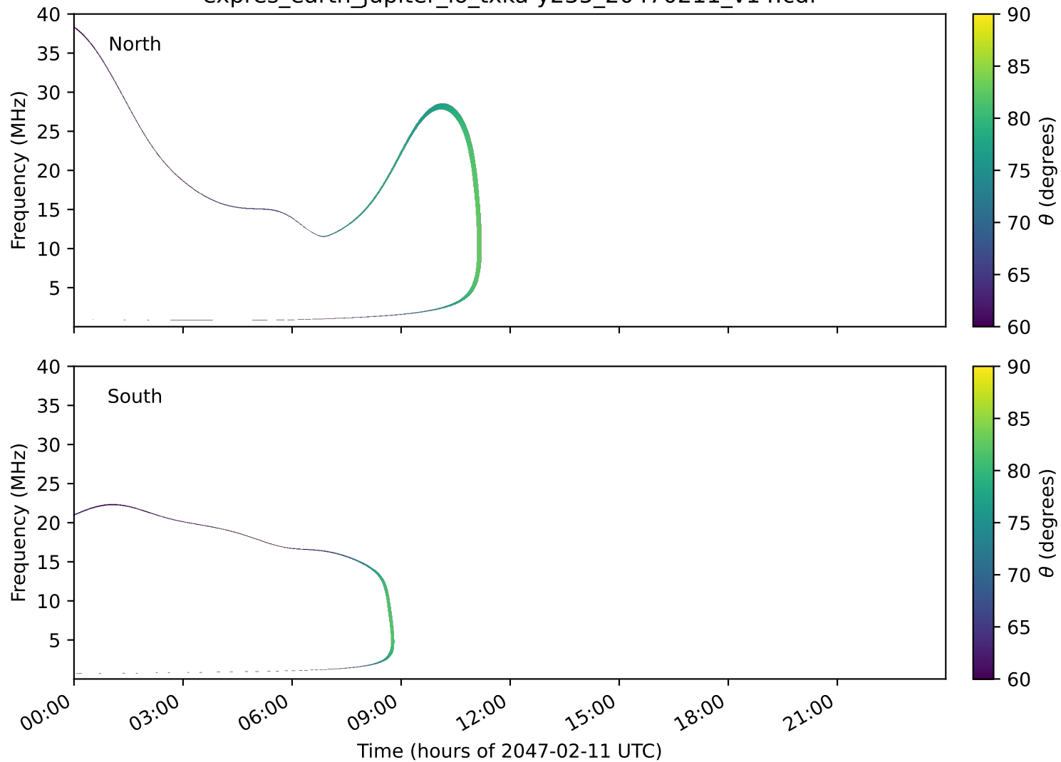
expres_earth_jupiter_io_txka-y235_20470211_v14.cdf
