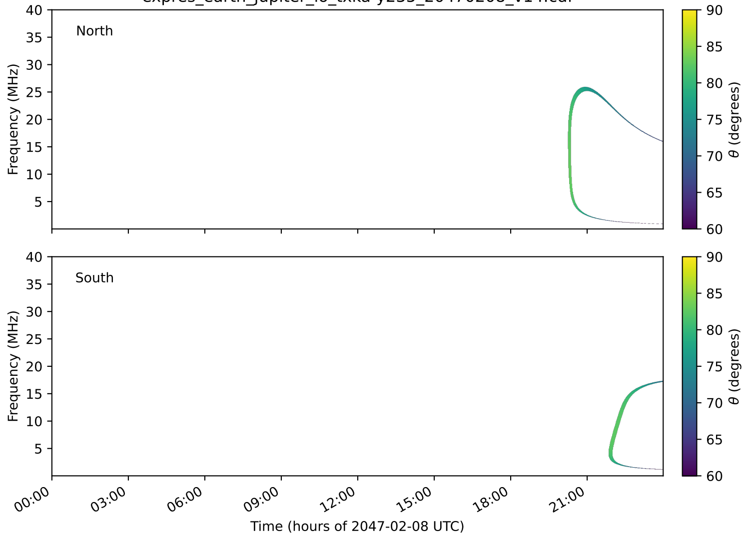
expres_earth_jupiter_io_txka-y235_20470208_v14.cdf
