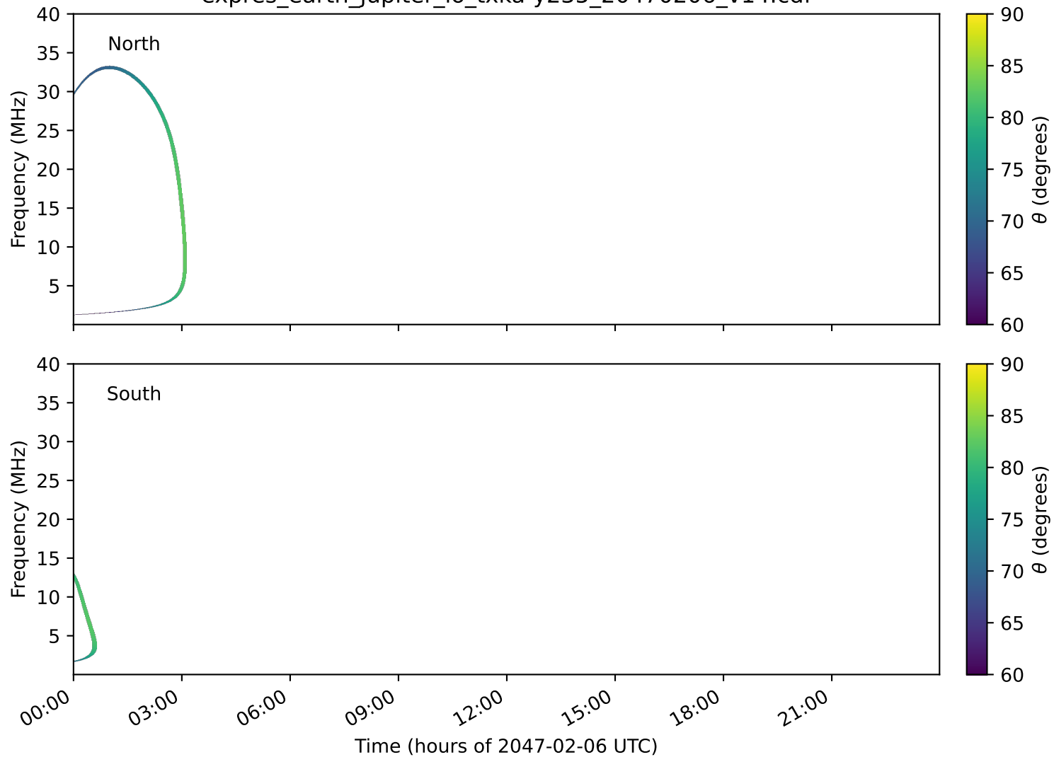
expres_earth_jupiter_io_txka-y235_20470206_v14.cdf
