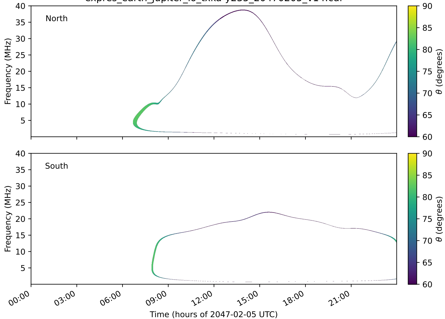
expres_earth_jupiter_io_txka-y235_20470205_v14.cdf
